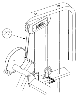
BELT ROUTING DETAIL
