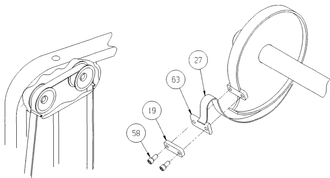
BELT ROUTING DETAILS
